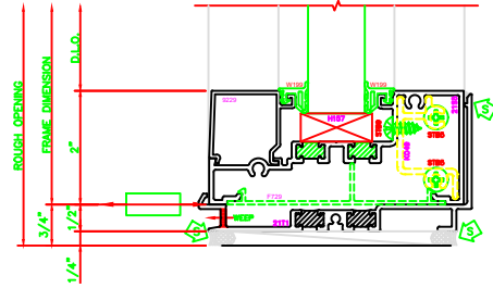
203 O.G. SILL SERIES: 403X - 2" X 4 1/2" SHEARBLOCK
